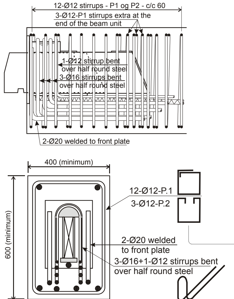
Figure 1 BSF 200/40, reinforcement in the beam end
