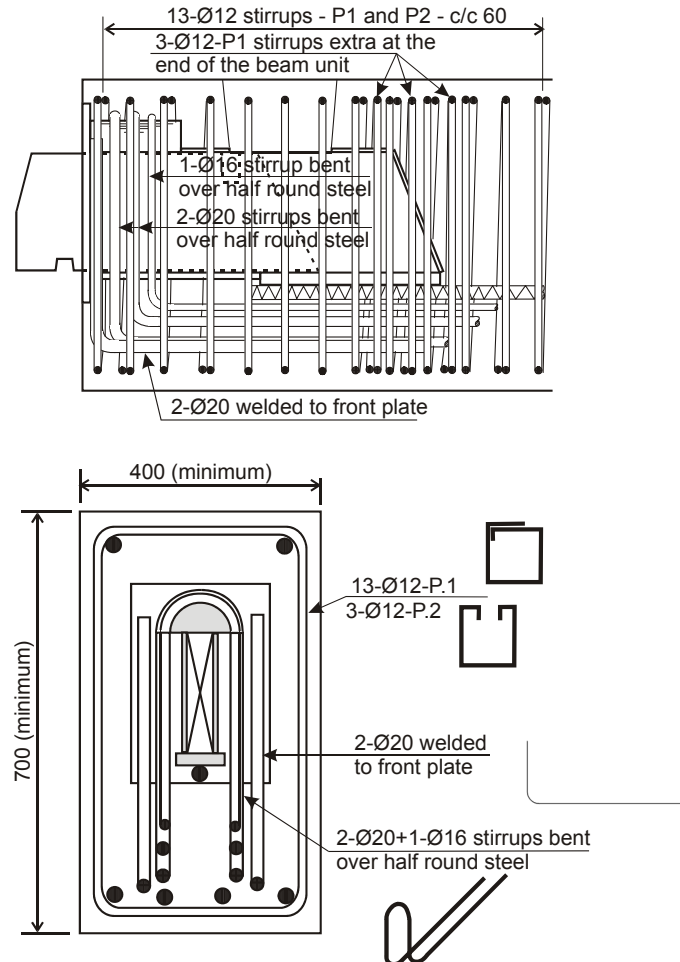
Figure 1 BSF 200/50, reinforcement in the beam end
