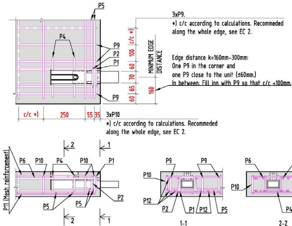
Figure 2: Recommended reinforcement pattern for RVK 41 units. Edge distance 160\text{mm} \leq k \leq 300\text{mm} . Ultimate limit load according to Figure 5.
