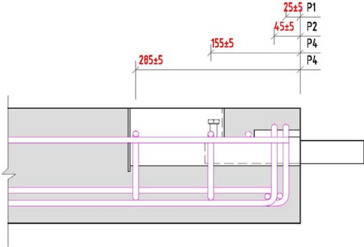
Figure 4: Tolerances P1, P2 and P4.
