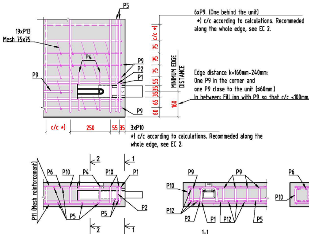
Figure 3: Recommended reinforcement pattern RVK 41. Slab thickness t < 200\text{mm} and edge distance 160\text{mm} \leq k \leq 240\text{mm} . Ultimate limit load according to Figure 5.
