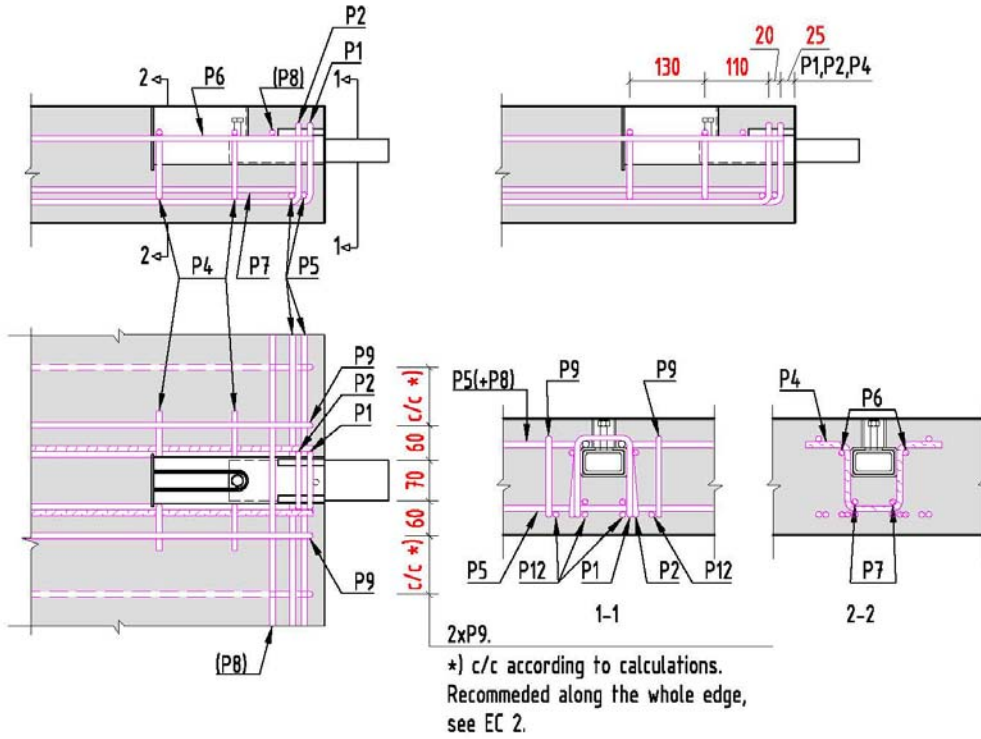
Figure 1: Recommended reinforcement pattern for RVK 41 units. Edge distance k > 300\text{mm} .
