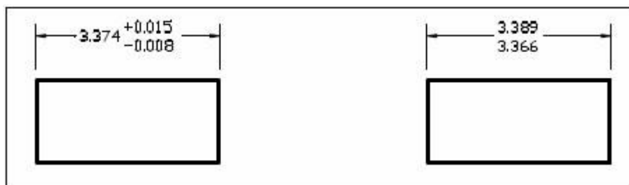
Tolerance dimension.
